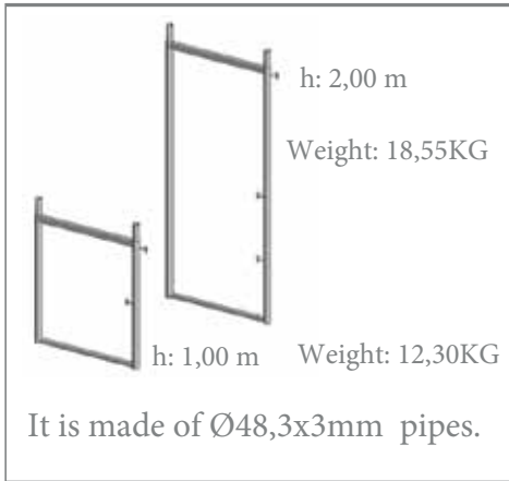
Guard Rail
